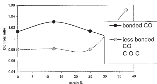
Figure 7: Sample A143 Plot of the dichroic ratio of carbonyl bands and ether band
