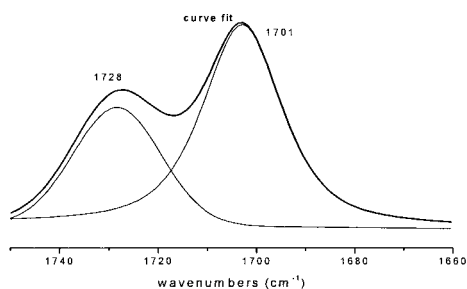
Figure 5: Deconvolved spectrum of A143
