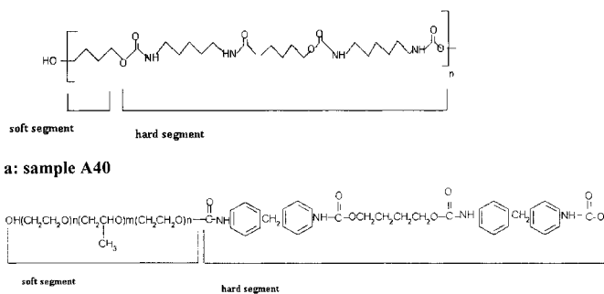
Figure 2: a) Sample A40 with the aliphatic hard segment and the amorphous soft segment. b) Sample A143 with the aromatic hard segment and the semicrystalline soft segment
