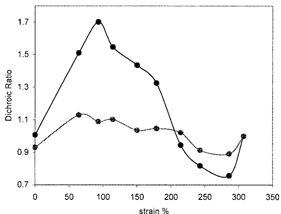
Figure 6: A40: Plot of the dichroic ratio as a function of % strain for the free and the hydrogen bonded carbonyl band
